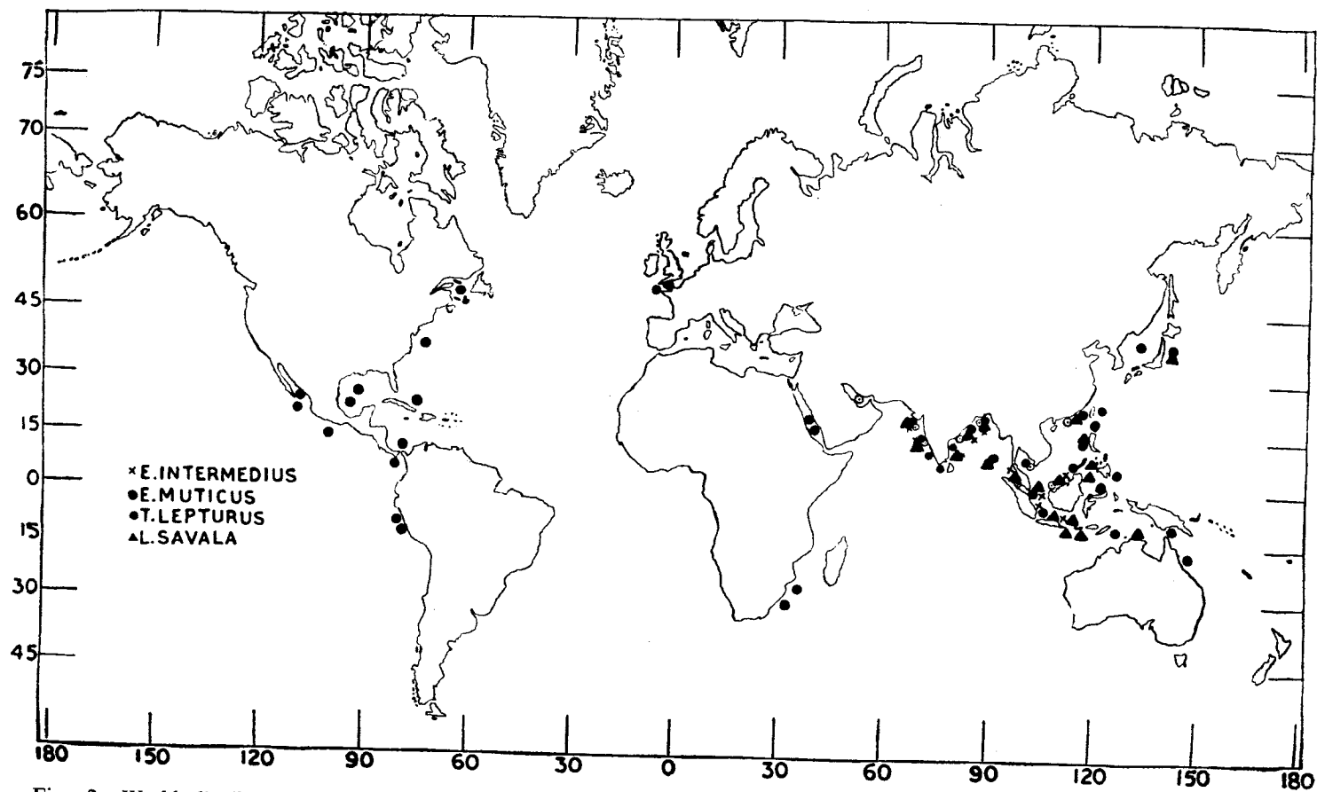
Fig. 2. World distribution of the four species of ribbon-fishes represented in Indian waters (the distribution of T. lepturus includes the distribution of all the species considered synonymous to it).
