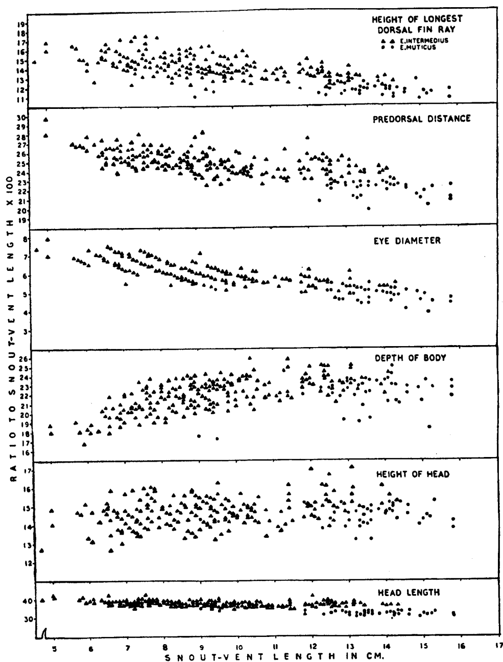
Fig. 5. Relative growth of body parts of E. intermedius and E. muticus .
