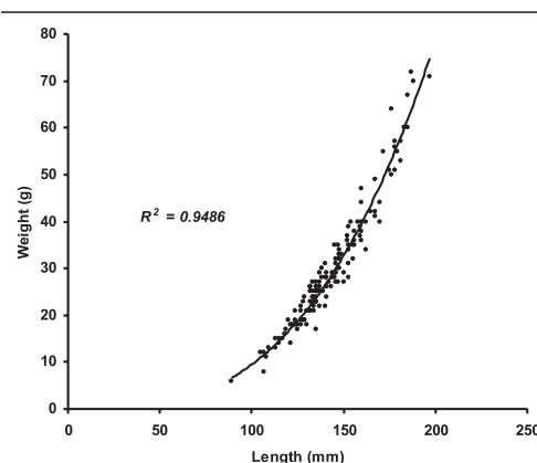
Fig. 3. Length-weight regression of T. myops (sexes pooled)
